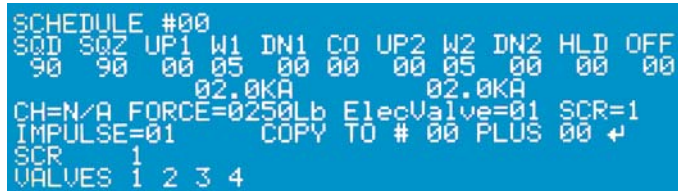
Force is part of the weld schedule.
